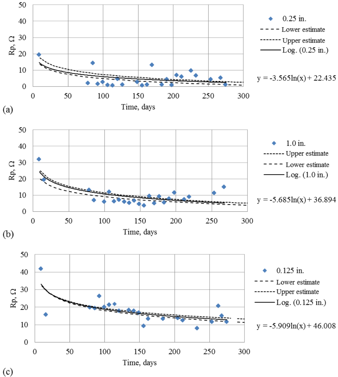
Figure 5.18 Linear polarization resistance (LPR) measurements at: (a) 0.25 inch concrete cover location, (b) 1.0 inch concrete cover location, and (c) 0.125 inch concrete cover location.
